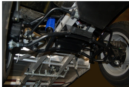
Newly Redesigned full tubular front suspension with adjustable coil over shocks.
