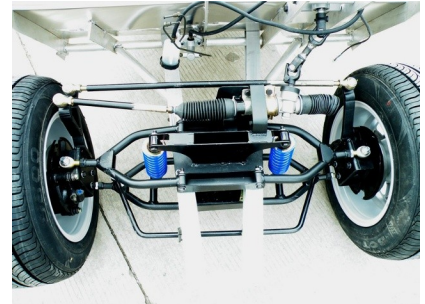
Shown here are more angles of the new suspension.
